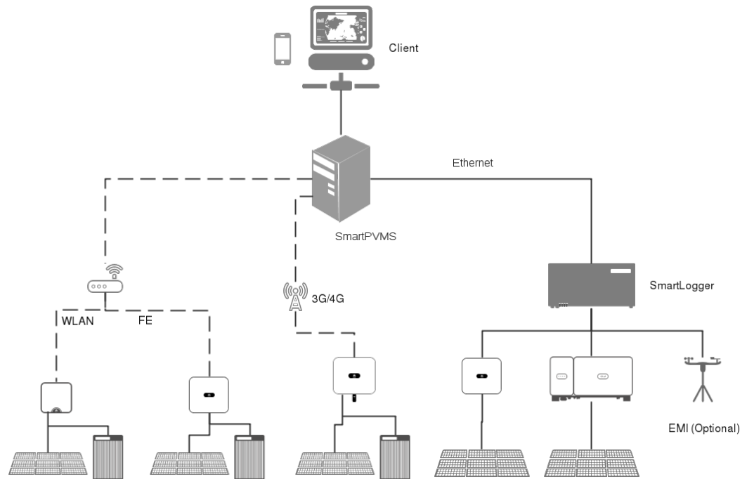
Figure 1-4 System networking
