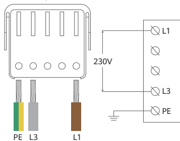
IT 1-phase
